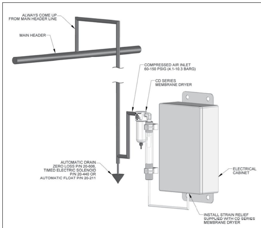
Figure 2: Recommended Installation
